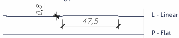
Internal lining profiles
