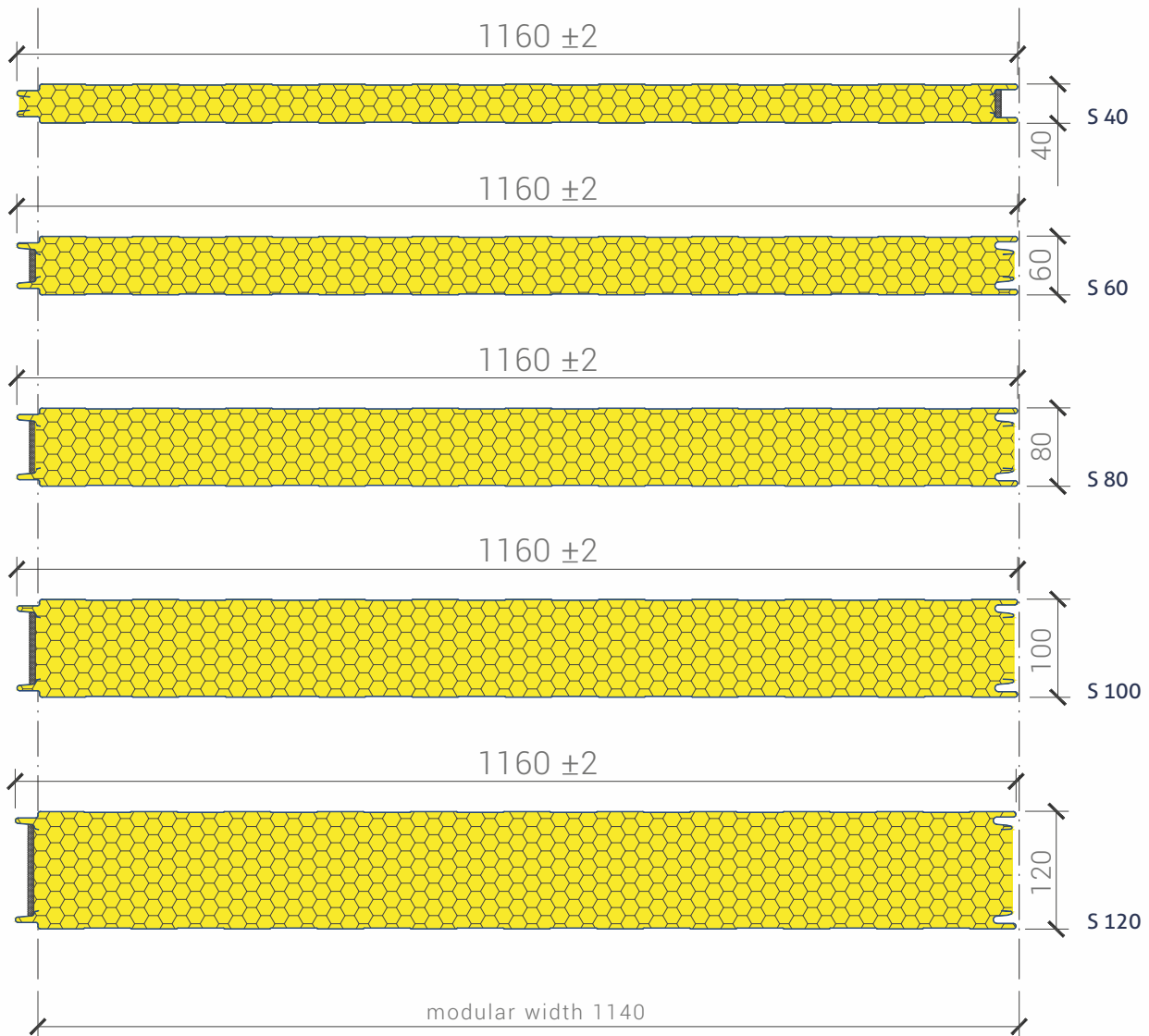
External lining profiles
