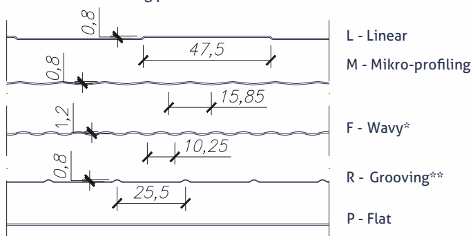
Internal lining profiles
