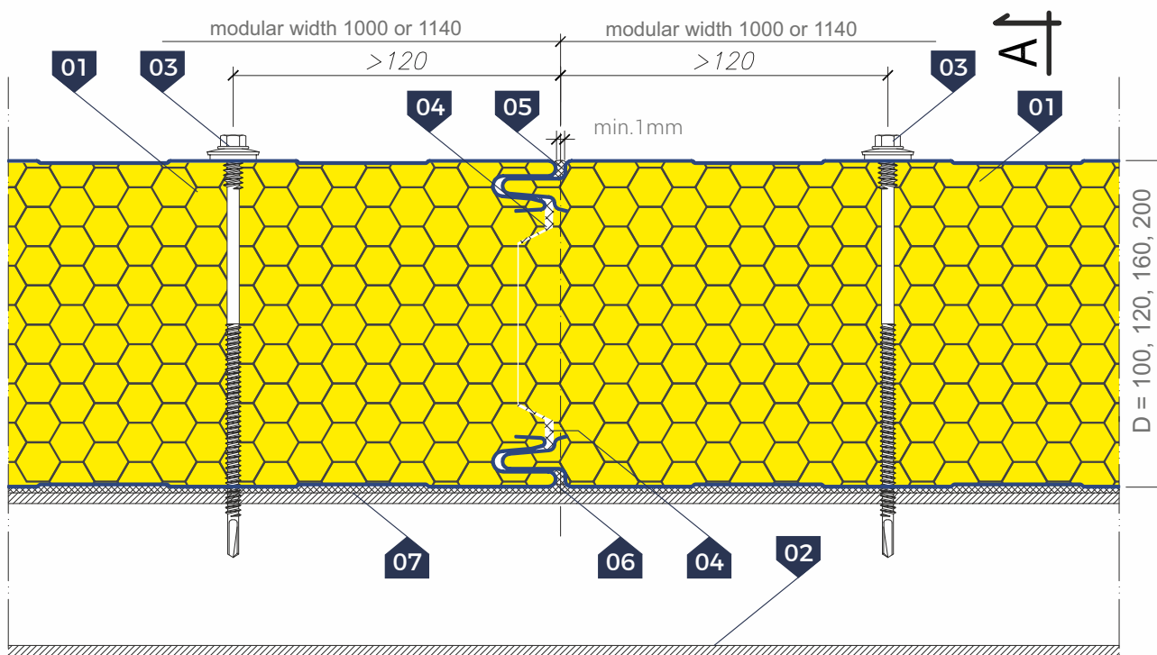
A-A cross-section
