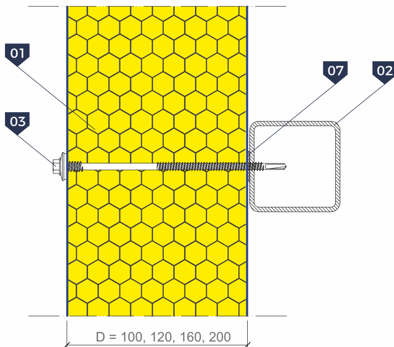
A-A cross-section
